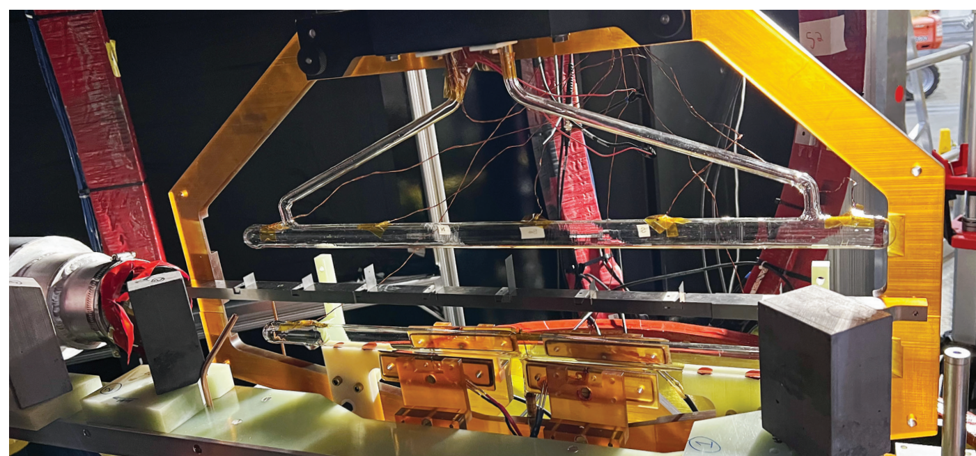
The polarized helium-3 target system with glass cells inside Experimental Hall A at Jefferson Lab.
